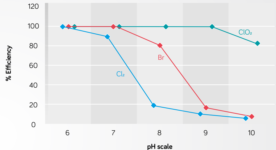
Comparison of the effectiveness of Chlorine, Bromine and Chlorine Dioxide between the pH range of 6-10
